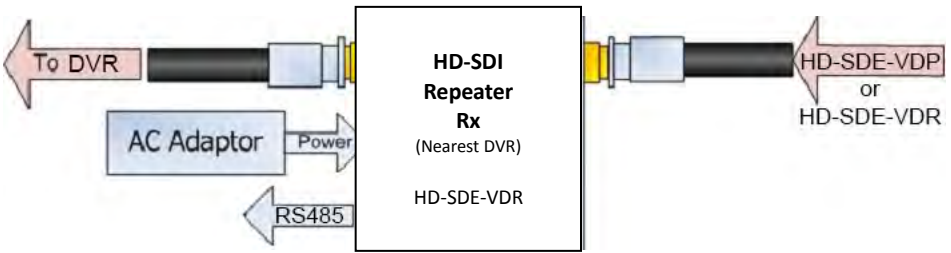
DVR/NVR side Repeater including Link Power and Control Channel
