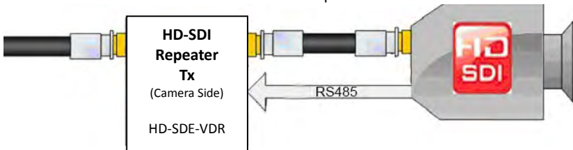
Camera side HD-SDI Repeater with Control
